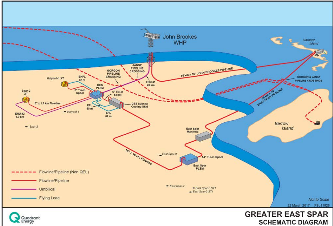
Figure 1-1: Greater East Spar Schematic
